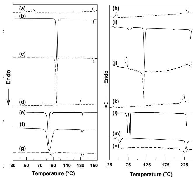
Fig. 1. DSC thermograms obtained with heating and cooling rates of 10 (a-d, f-i, k, m) or 20 °C/min (e, j, l, n): dash-line: 1st cooling; solid-line: 1st heating; dash-dot-line: 2nd heating. (a-c) 4a ; (d-g) 4b ; (h-j) 4c ; (k-n) 4d .
