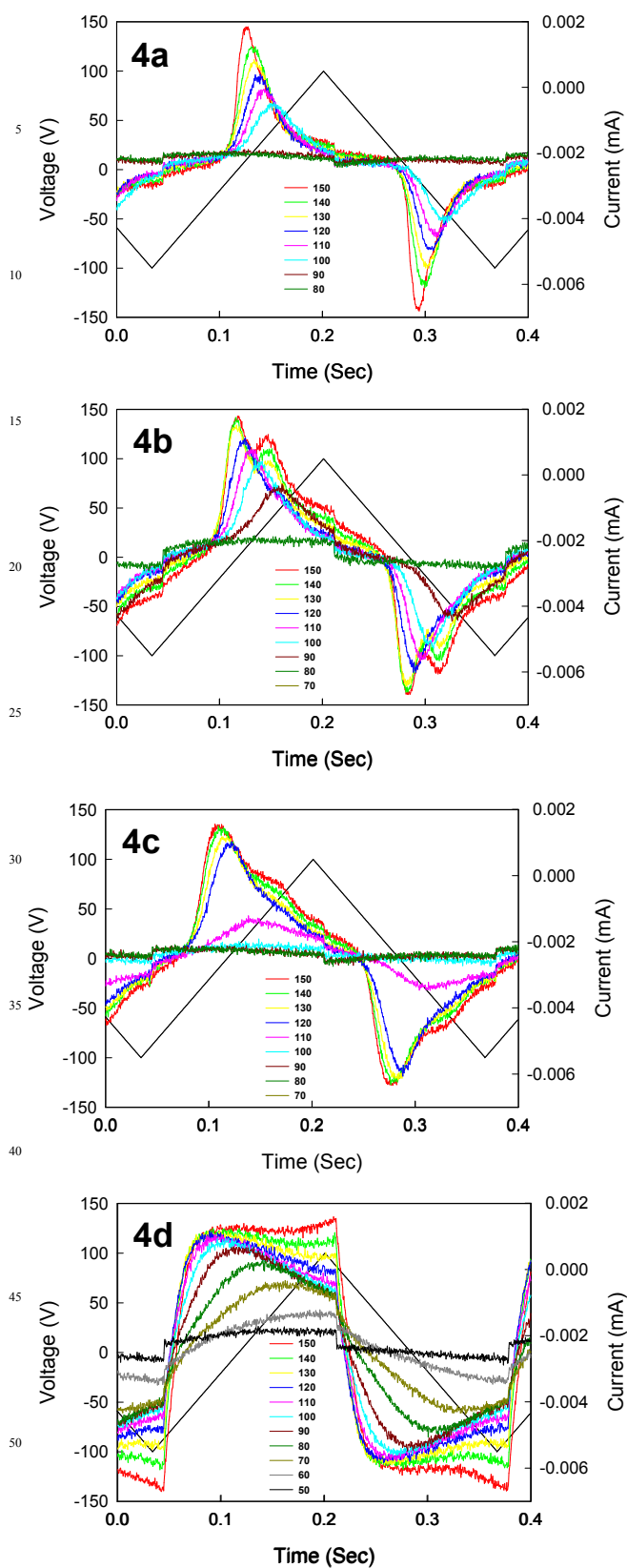
Fig. 5. Switching current response for compounds by applying a triangular voltage ( E = 22 \text{ V } \mu\text{m}^{-1} , f = 3 \text{ Hz} ) at given temperatures.
