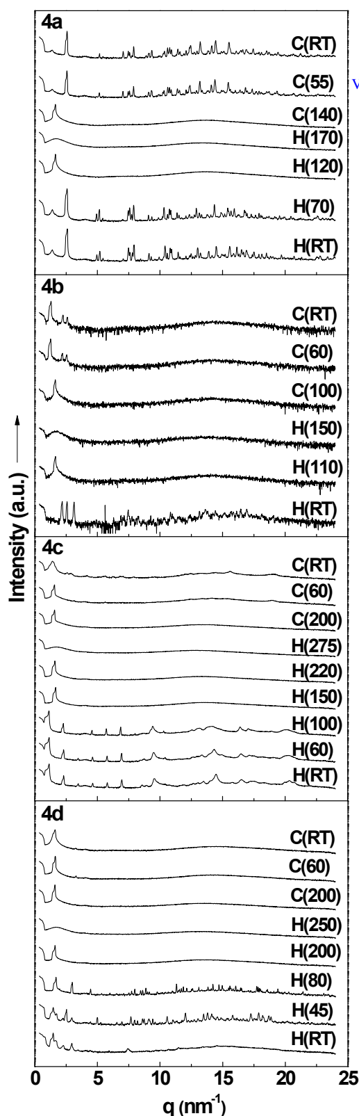
Fig. 2. Synchrotron radiation X-ray diffraction profiles of compounds obtained at given temperatures (°C, in parentheses). Abbreviation: RT = room temperature; H = heating process; C = cooling process.
