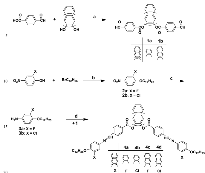
Scheme 1. Synthetic route to compounds: a) DCC, DMAP, \text{CHCl}_3 , rt, 24 h; b) \text{Na}_2\text{CO}_3 , DMF, reflux, 4 h; c) 100 psi \text{H}_2 , 10% Pd-C, EtOH, 70 °C, 4 h; d) EtOH, 80 °C, reflux, 8 h.
