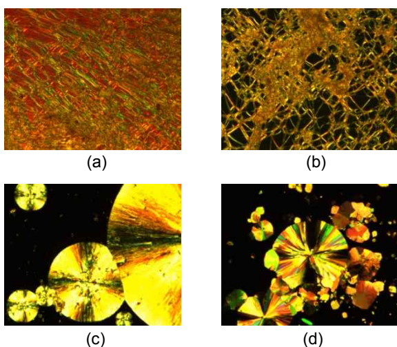
Fig. 3. Cross-polarizing optical micrographs obtained at given temperature (x200). On heating: (a) 4a , at 127°C; (b) 4d , at 225°C. On cooling: (c) 4a , at 37°C; (d) 4c , at 65°C.
